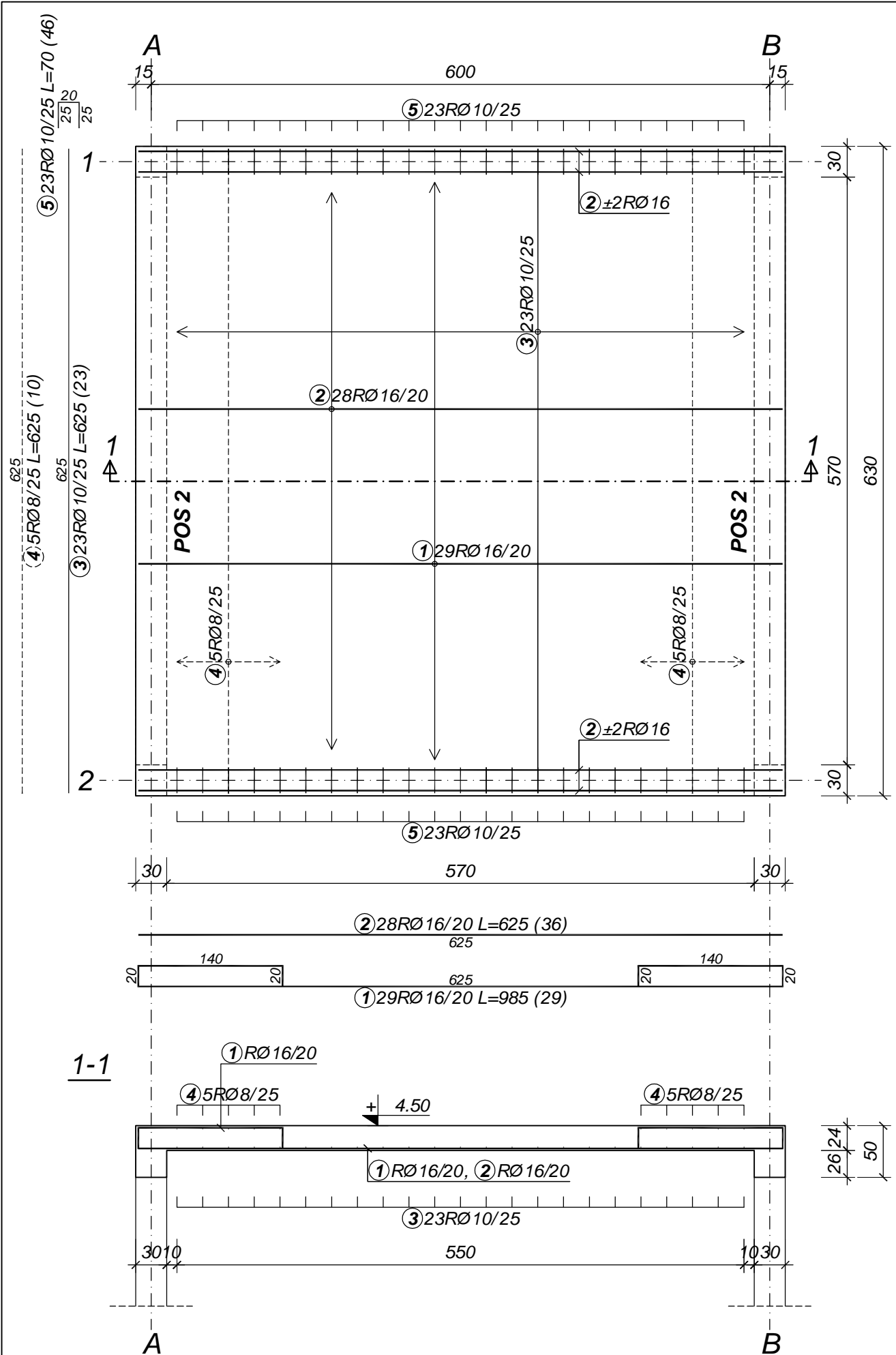
PLAN ARMATURE POS 1
